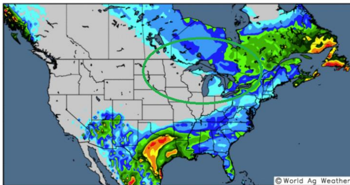
GFS High-Resolution Precipitation Forecast Days 1-7: 00UTC 16 Oct 2018 - 00UTC 23 Oct 2018 Model Initialized 00UTC 15 Oct 2018
