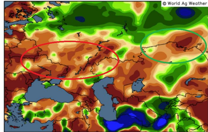
14-day Precipitation Analysis Percent of normal through 14 Oct 2018
