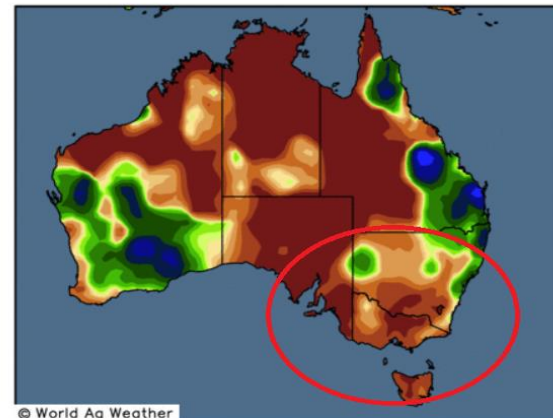
30-day Precipitation Analysis Percent of normal through 14 Oct 2018
