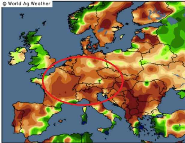
30-day Precipitation Analysis Percent of normal through 14 Oct 2018
